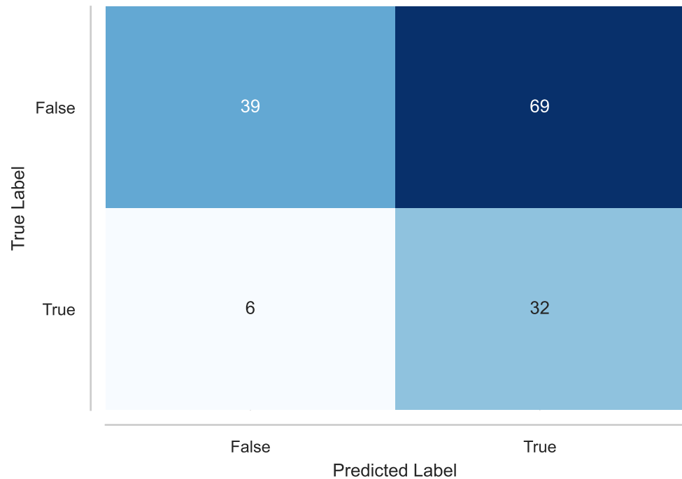
Confusion Matrix - SVC
